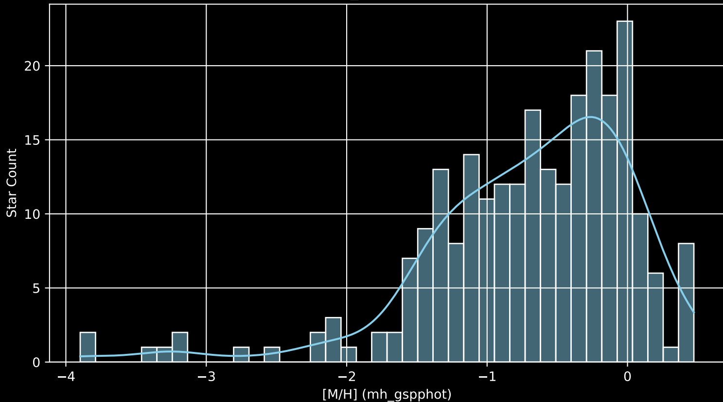
APOGEE DR17 Field: [206-02-C [M/H] (mh_gspphot) (n= 251)
