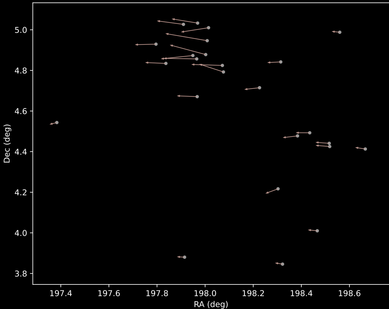
APOGEE DR17 Cluster 11 Proper Motion Vectors (n=25)
