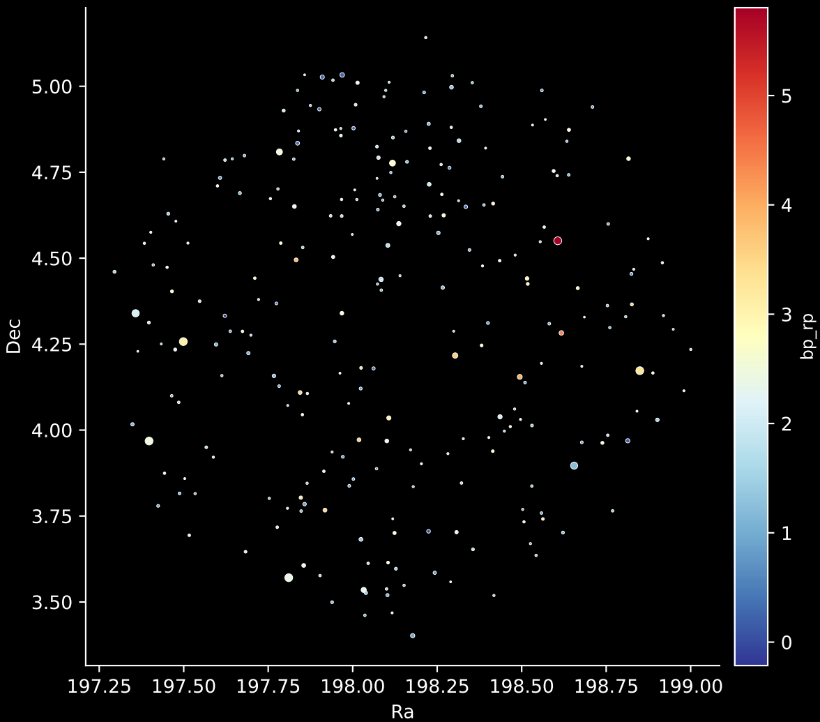
APOGEE DR17 Field: [206-02-C] Stars: 254
