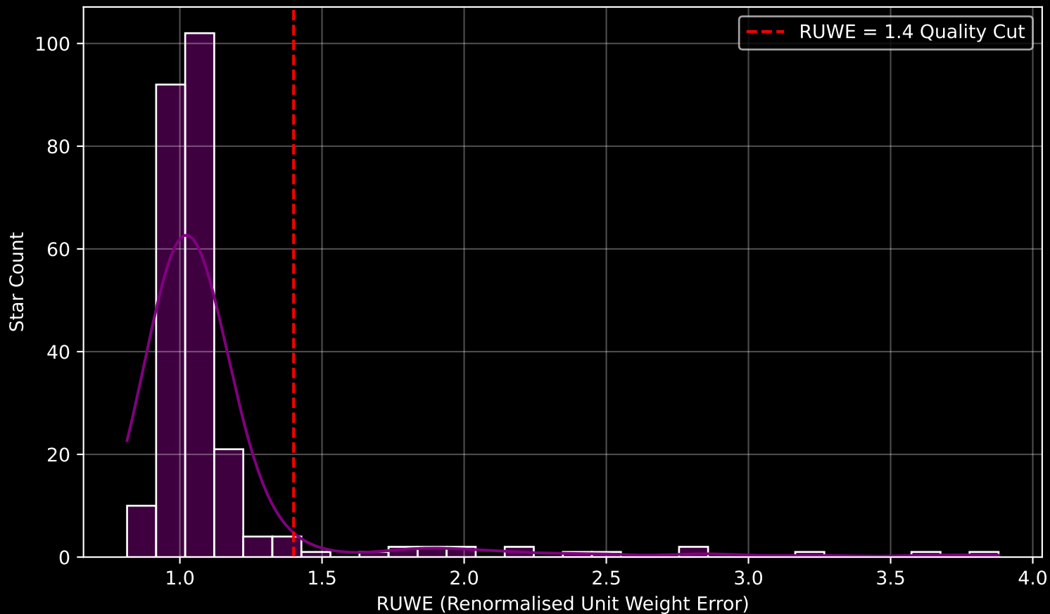
GAPOGEE DR17 Field [206-02-C] RUWE Distribution (n= 250)
