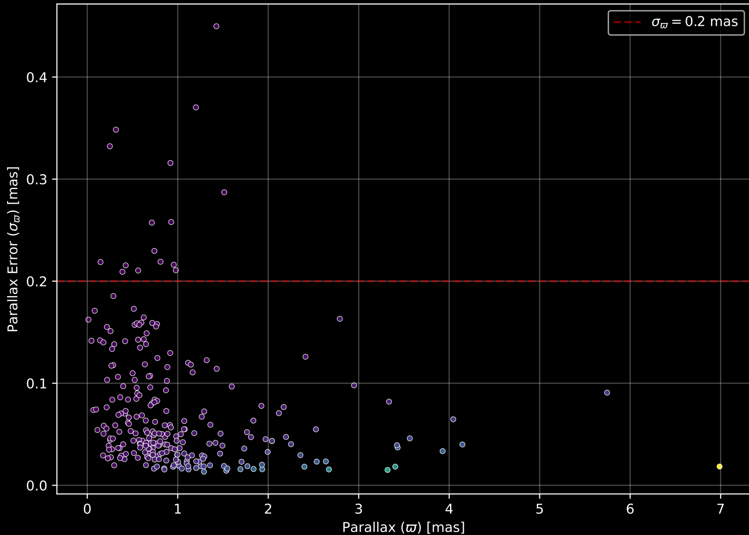
APOGEE DR17 Field: [206-02-C] Parallax Quality (n= 254)
