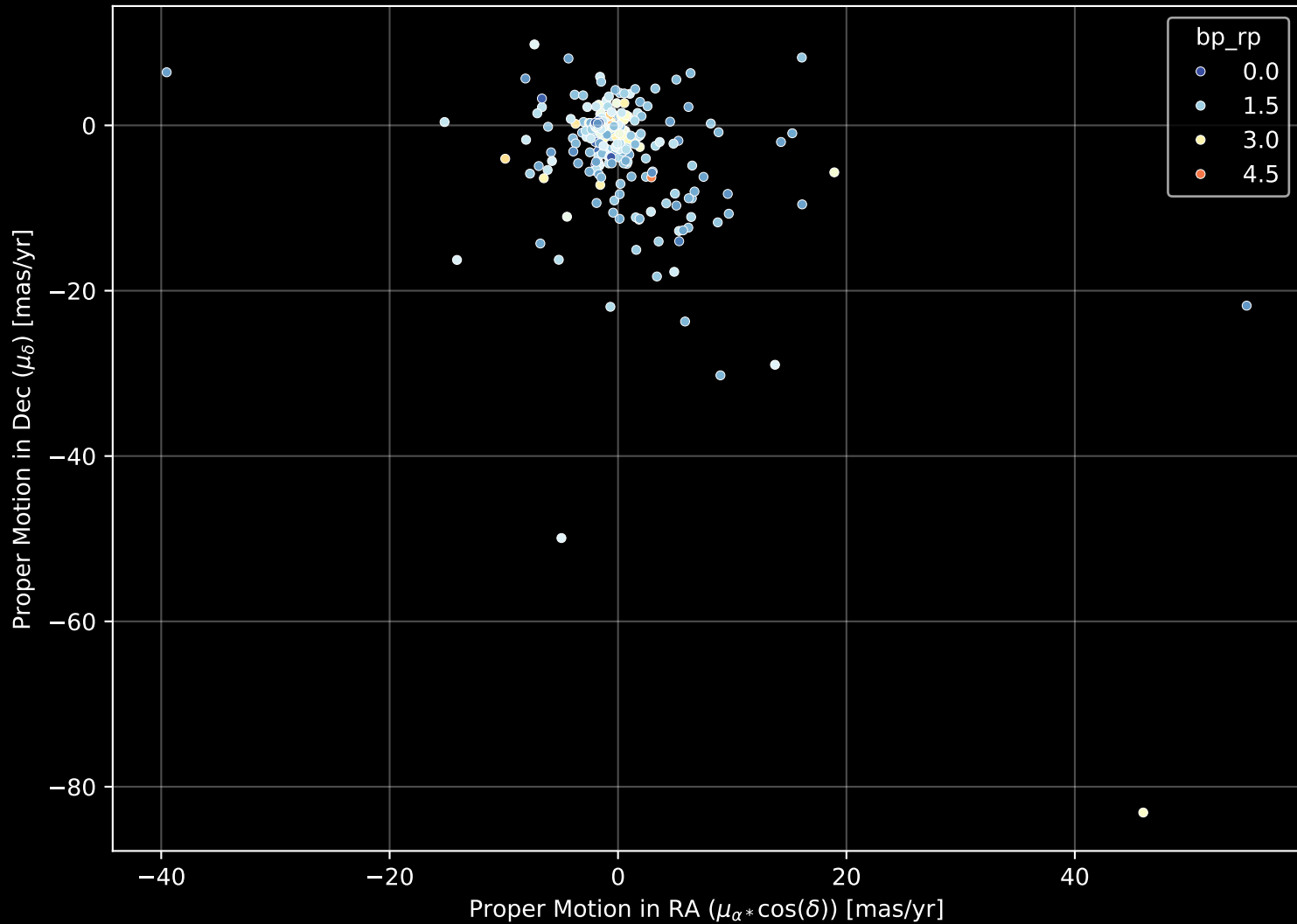
APOGEE DR17 Field: [206-02-C] Proper Motion Diagram (n= 254)
