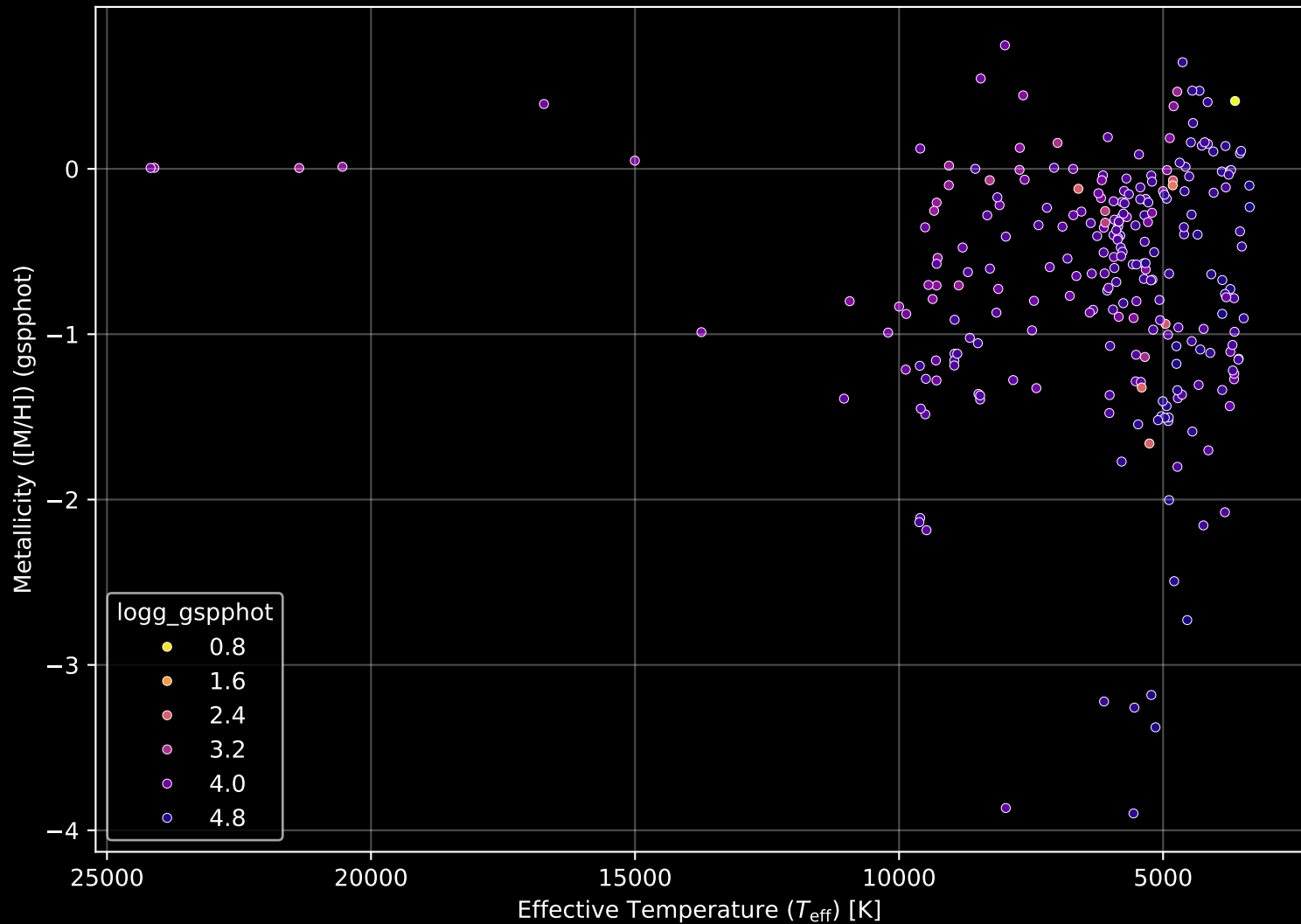
APOGEE DR17 Field: [206-02-C] Stellar Population Parameters (n= 254)
