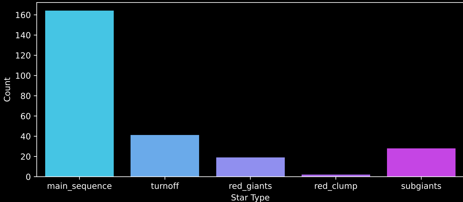
APOGEE DR17 Field: [206-02-C] Count plot of Star Type
